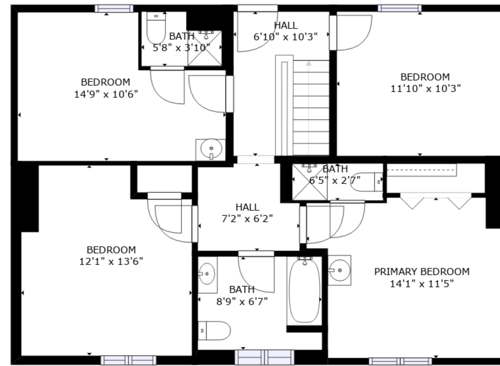
FLOOR 3
